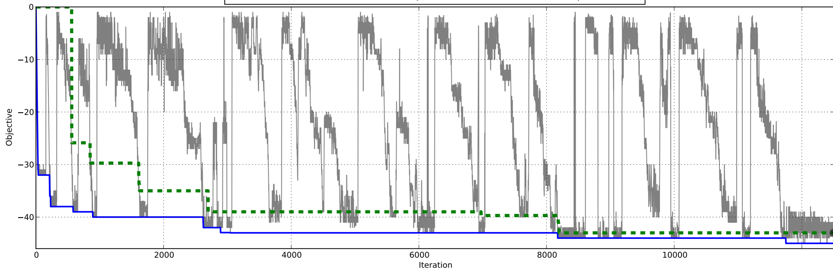
— Incumbent solution — Best partial solution — Best complete solution
